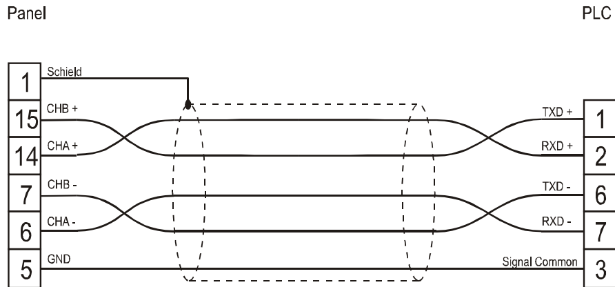
figure 1. Cable diagram
