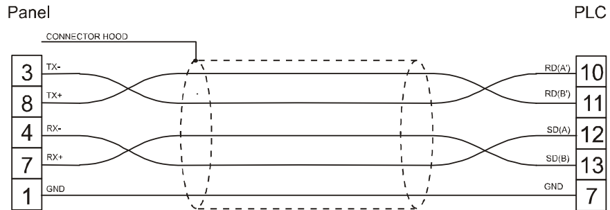
figure 1. Cable diagram
