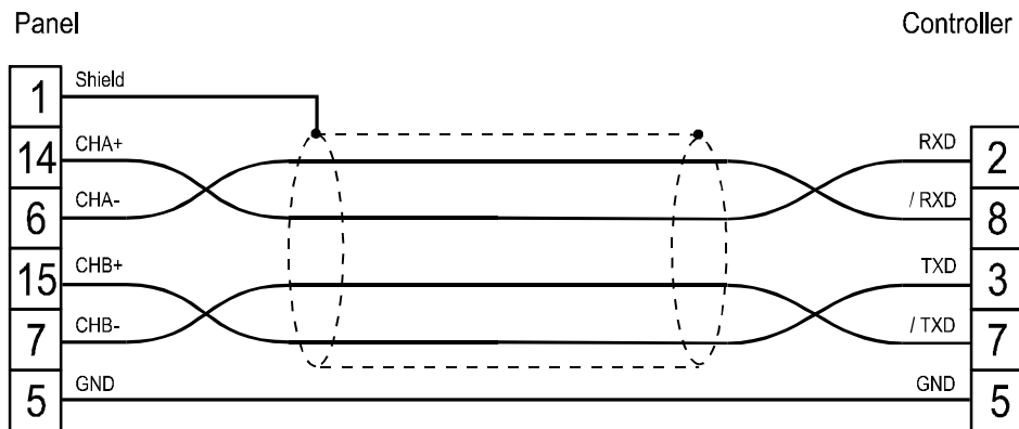
Figure 1. Cable diagram
