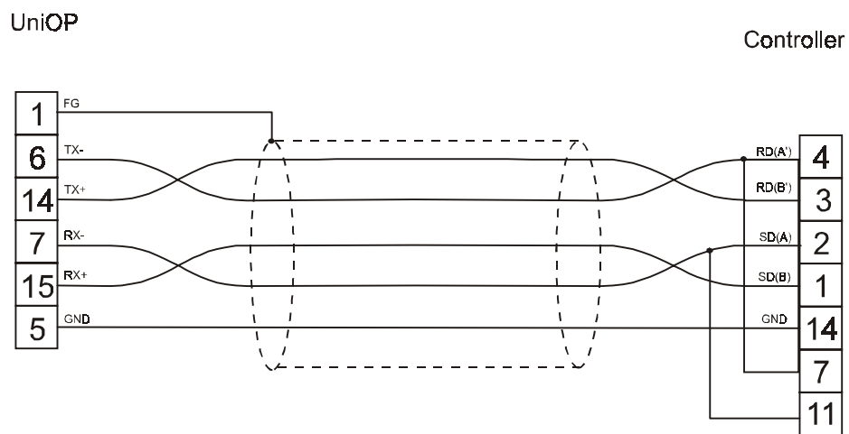
figure 1. Cable diagram
