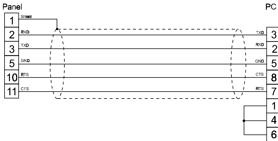
figure 1. Cable diagram
