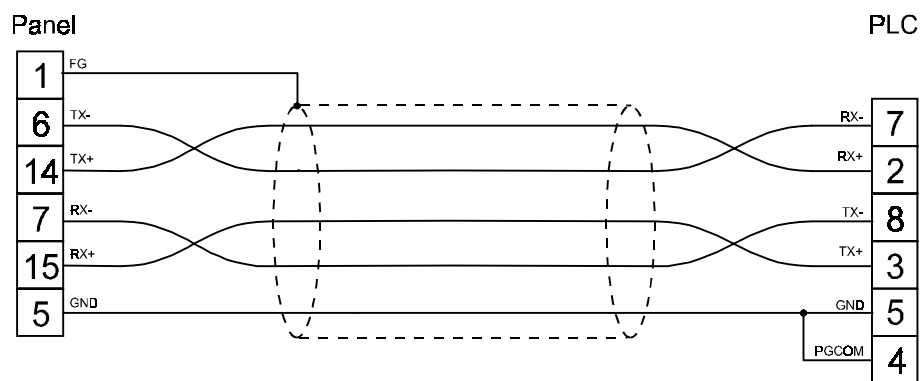
figure 1. Cable diagram
