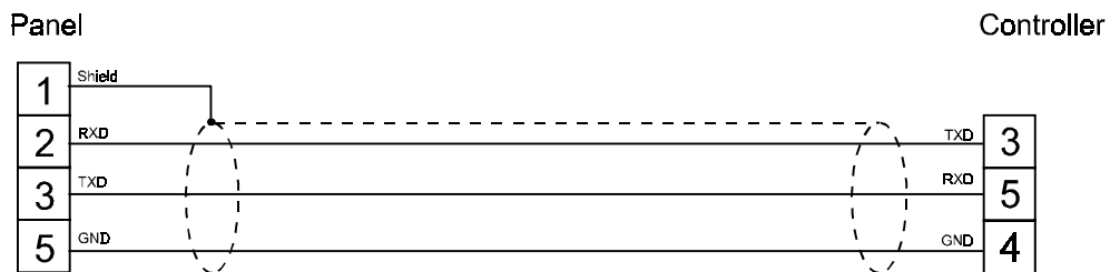
figure 1. Cable diagram
