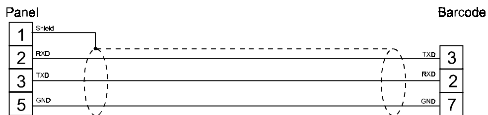
figure 1. Cable diagram
