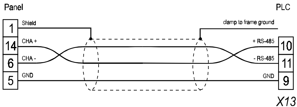
figure 1. Cable diagram
