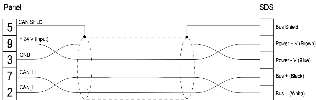
Figure 1. Cable diagram
