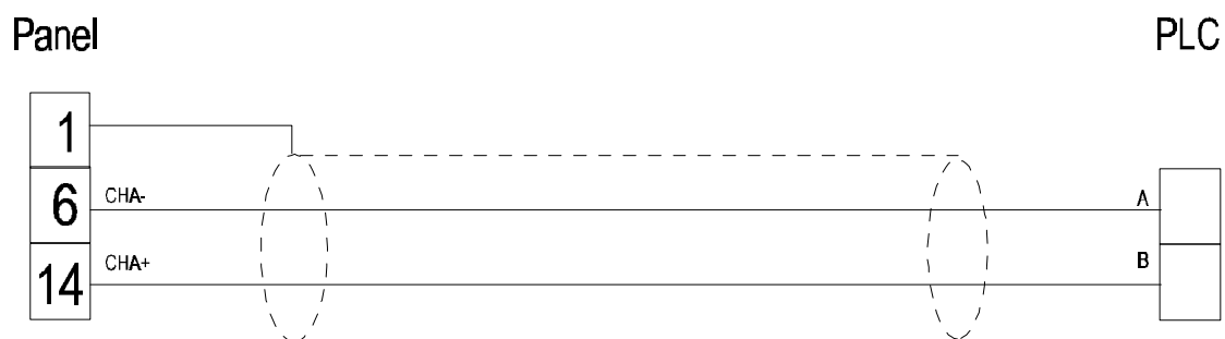
Figure 1. Cable diagram
