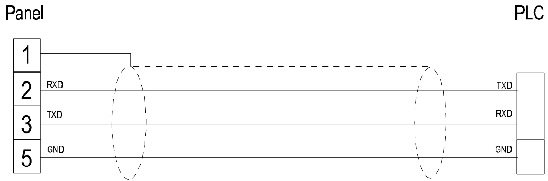
Figure 1. Cable diagram
