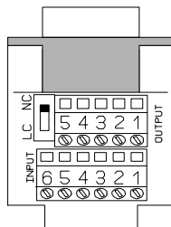
Figure 1 – Connector view (IB-ADP adapter)
