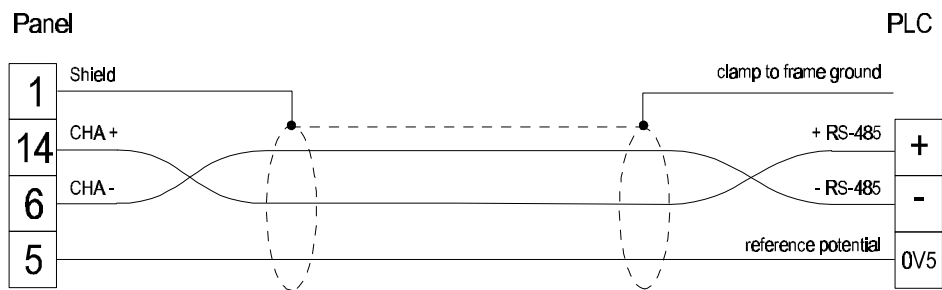
figure 1. Cable diagram
