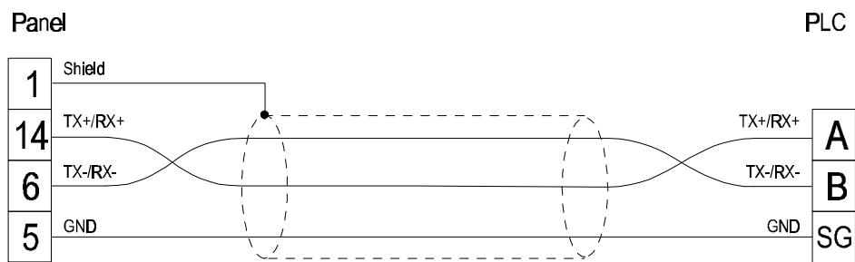
figure 1. Cable diagram
