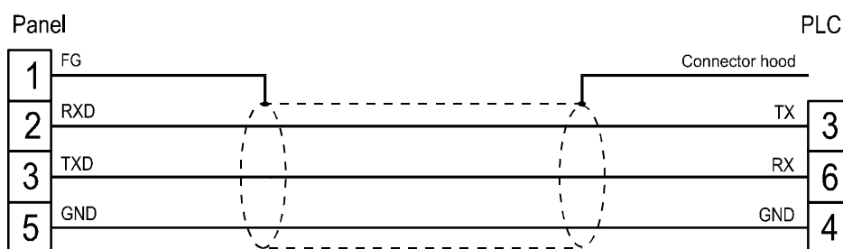
Figure 1. Cable diagram
