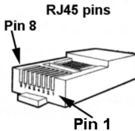
Figure 2. PLC connector
