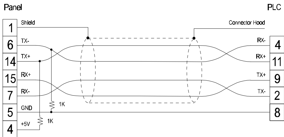
Figure 1. Cable diagram
