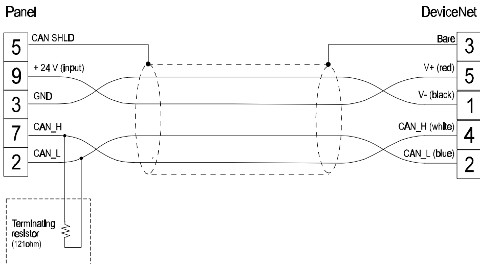
Figure 1. Cable diagram
