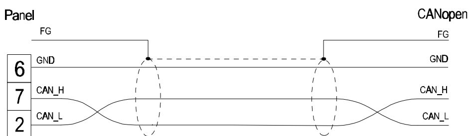
Figure 1. Cable diagram
