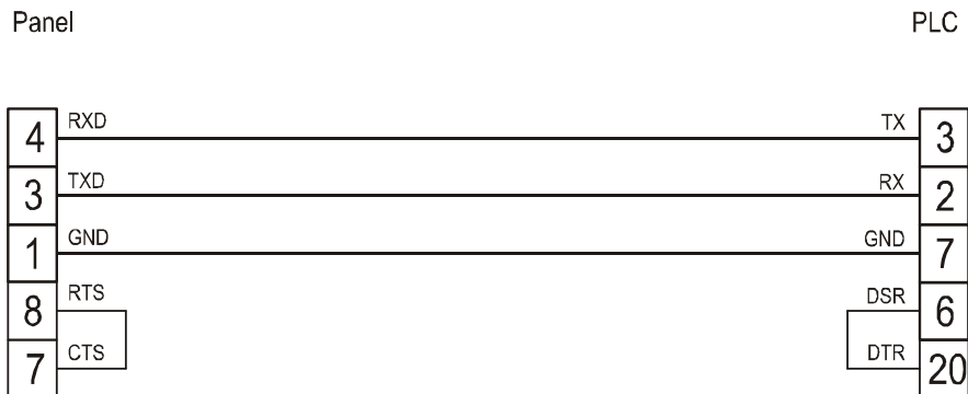
Figure 1. Cable diagram
