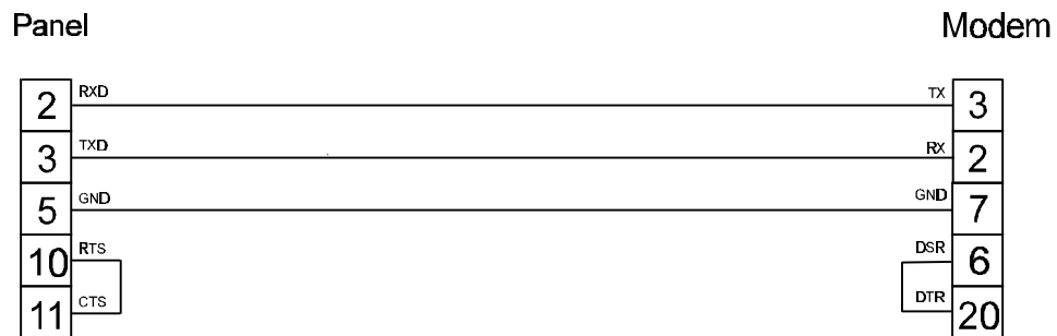
figure 1. Cable diagram
