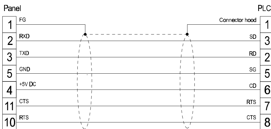
Figure 1. Cable diagram
