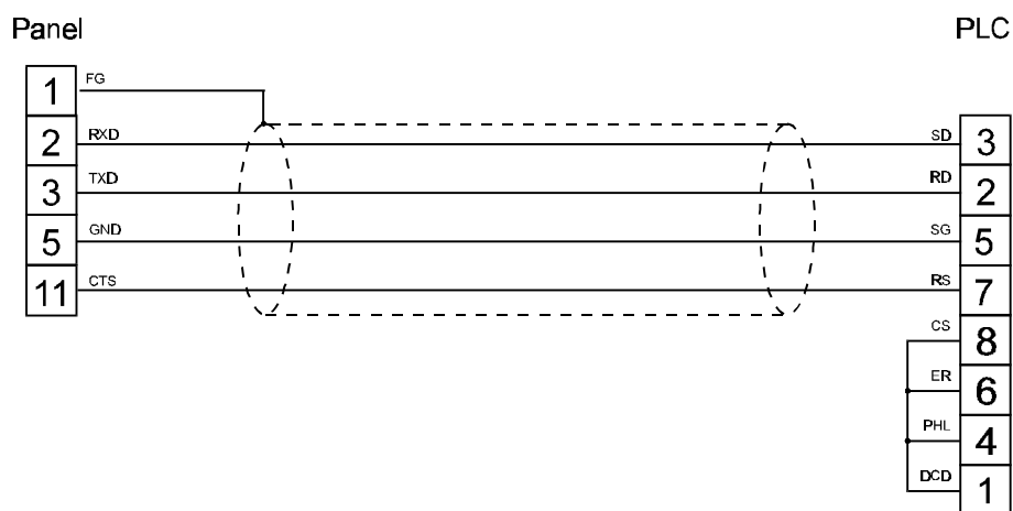
figure 1. Cable diagram
