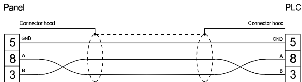
figure 1. Cable diagram
