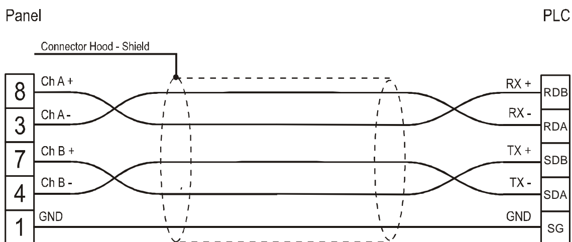
Figure 1. Cable diagram
