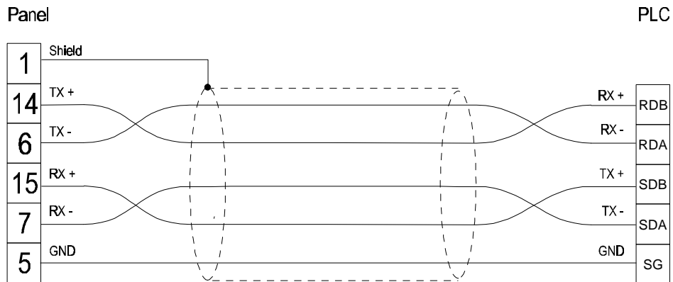
Figure 1. Cable diagram
