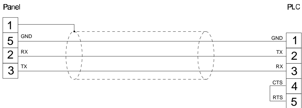
Figure 1. Cable diagram
