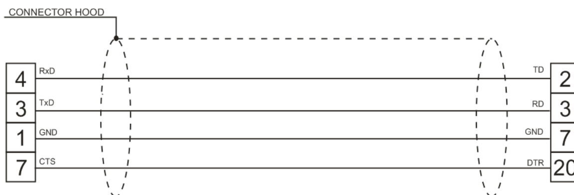
Figure 1. Cable diagram
