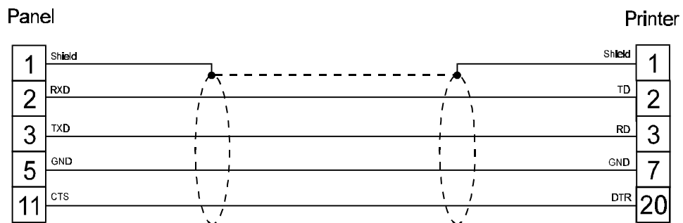
figure 1. Cable diagram
