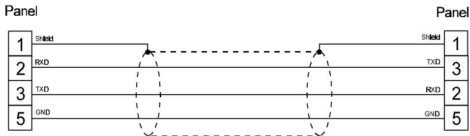
figure 1. Cable diagram
