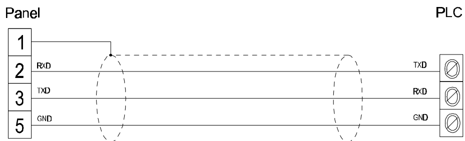
Figure 1. Cable diagram
