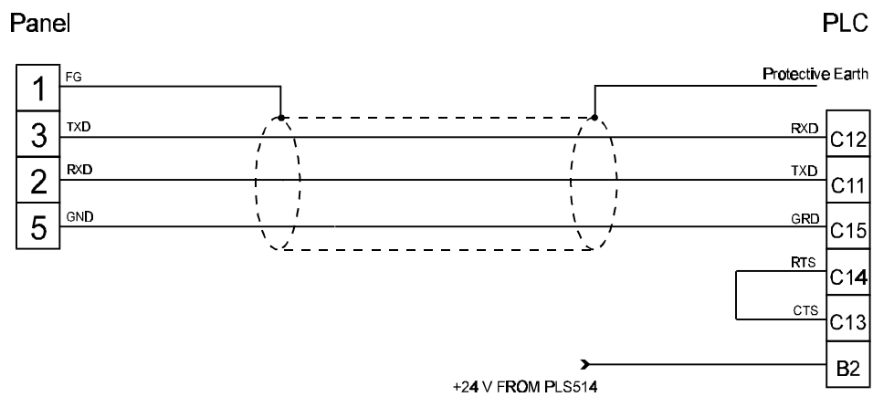
figure 1. Cable diagram
