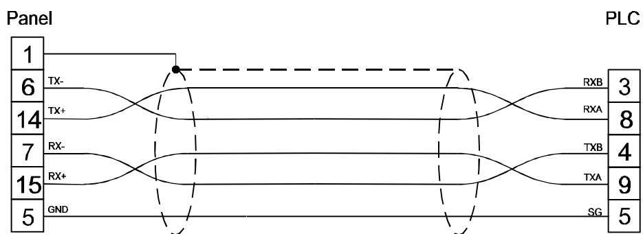
figure 1. Cable diagram
