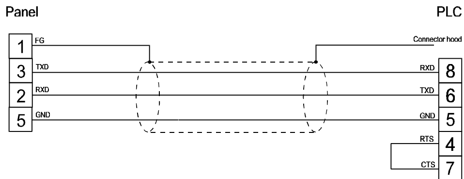
figure 1. Cable diagram
