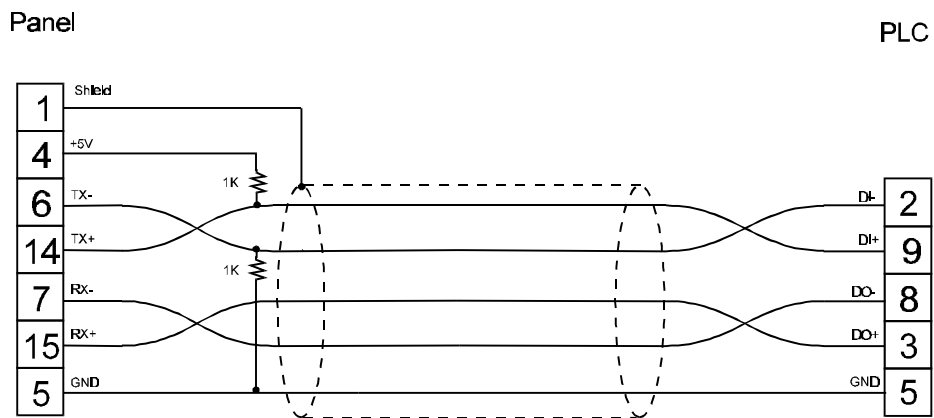
figure 1. Cable diagram
