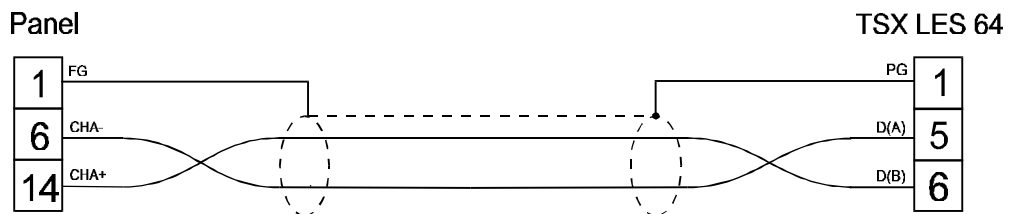
figure 1. Cable diagram
