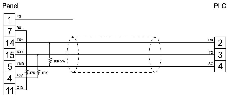
figure 1. Cable diagram
