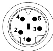
Figure 2. PLC connector
