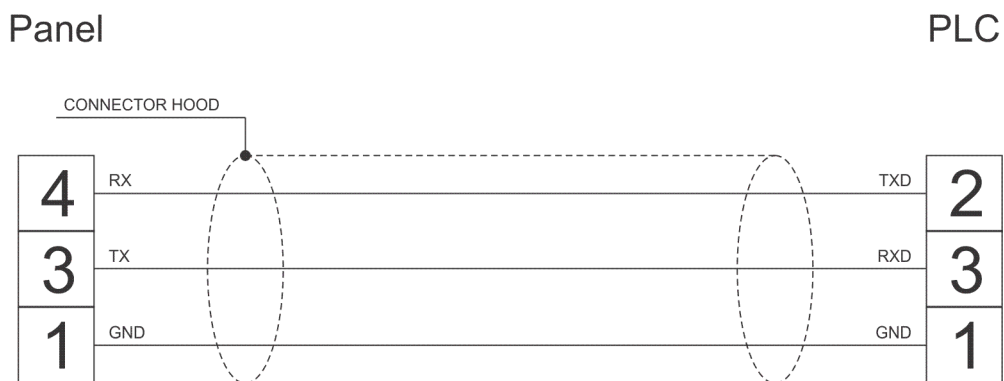
Figure 1. Cable diagram
