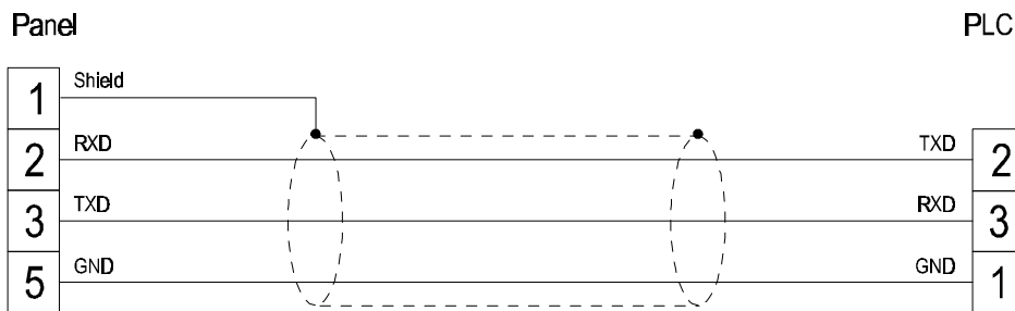
Figure 1. Cable diagram
