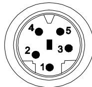
Figure 2. PLC connector
