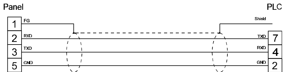
figure 1. Cable diagram
