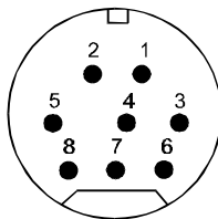
figure 2. Connector front view (pin side)
