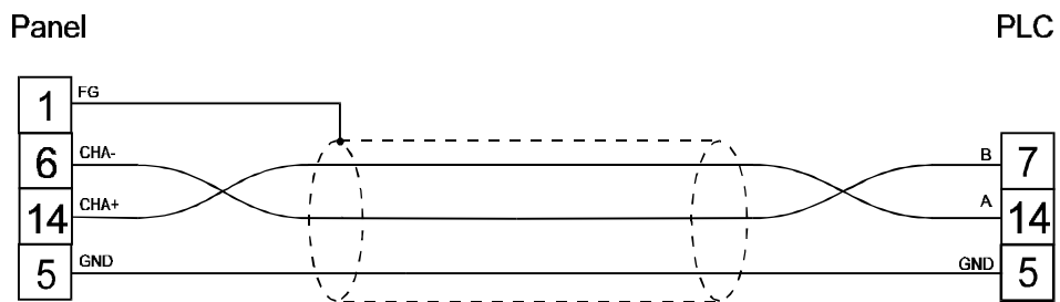
figure 1. Cable diagram
