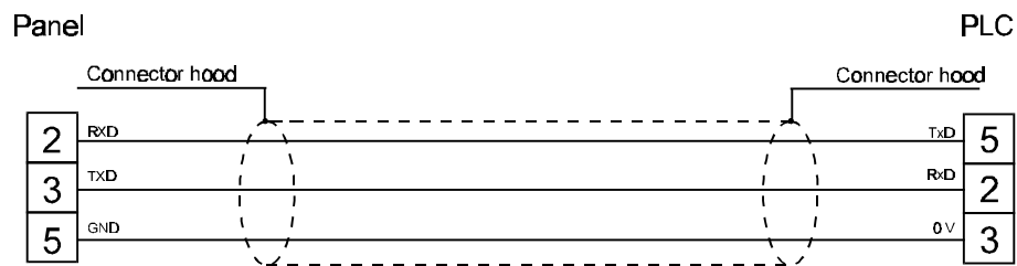
Figure 1. Cable diagram
