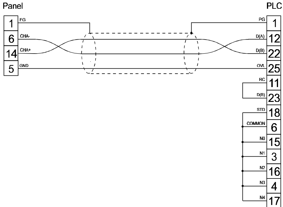
figure 1. Cable diagram
