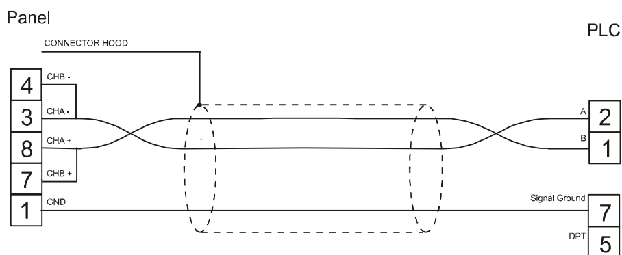
figure 1. Cable diagram
