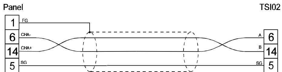
figure 1. Cable diagram
