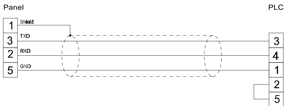
Figure 1. Cable diagram
