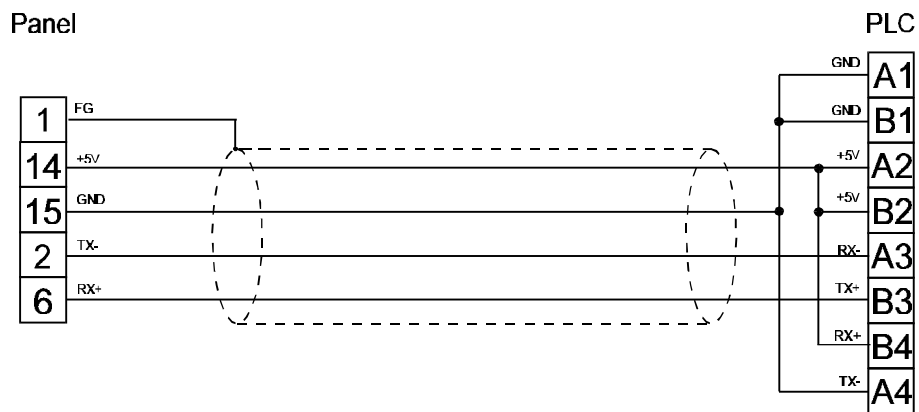
figure 1. Cable diagram
