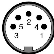
figure 2. Connector front view (pin side)
