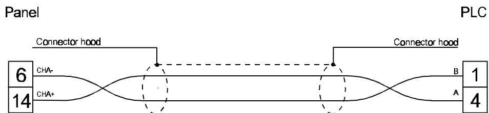
figure 1. Cable diagram
