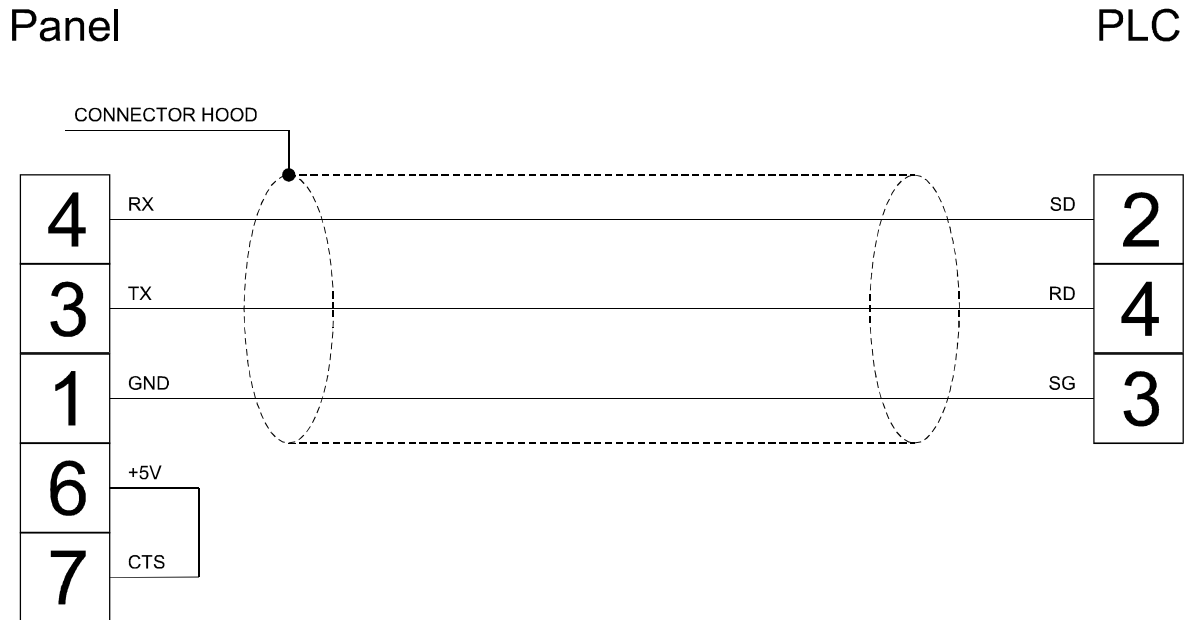
figure 1. Cable diagram
